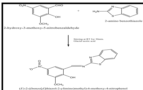
Fig. 1 Synthesis of Schiff base ( S_5 ) ligand
