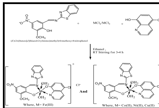
Fig. 2 Synthesis of mixed ligand complexes
